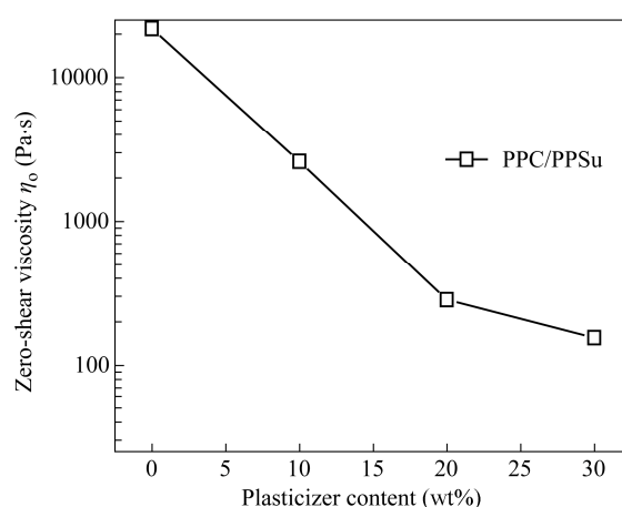
Fig. 8 Effect of plasticizer content on the zero-shear viscosity of PPC/PPSu blends at 160 °C
